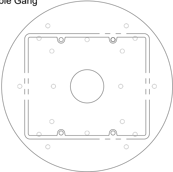
Double Gang
